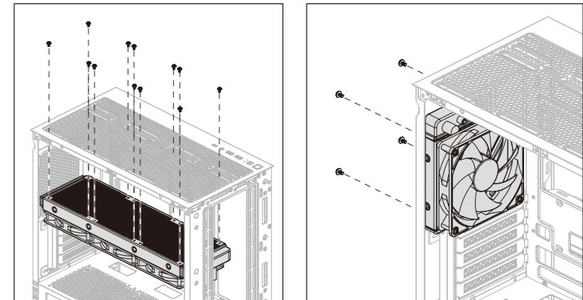
(6b) Install Top Radiator
