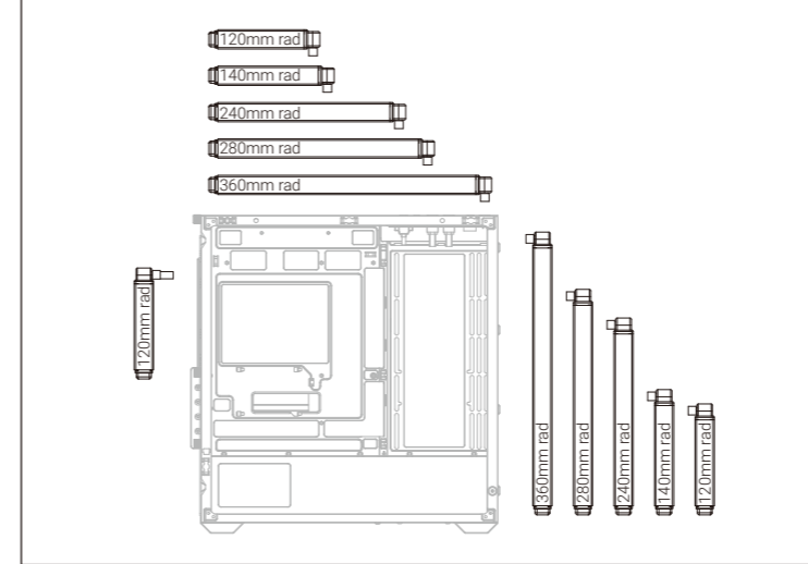
Radiator Support
