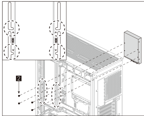
(4b) Install 3.5" HDD x1
