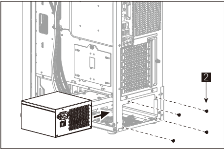
(2) Install Power Supply Unit
