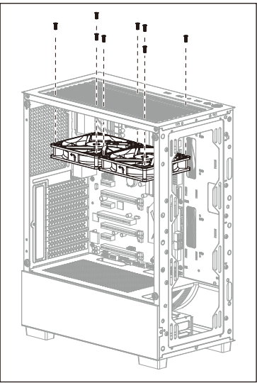
(7d) Install Top Fans
