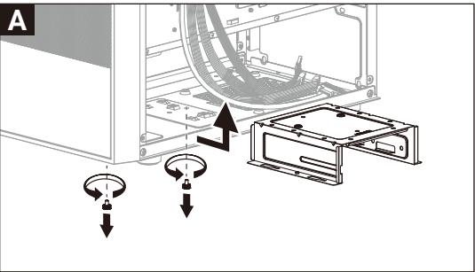
(4) Install 3.5" HDD x2
