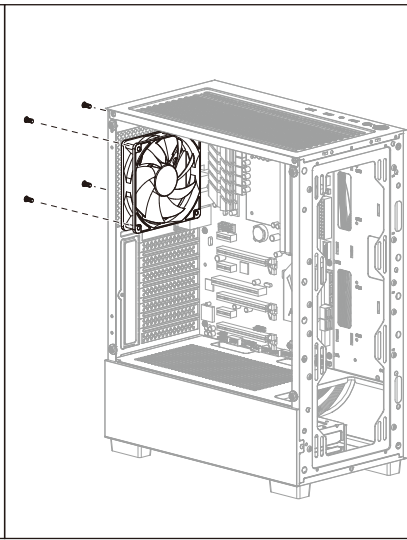
(7c) Install Rear Fans
