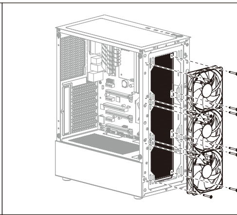
(7b) Install Front Fans
