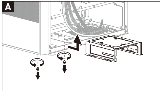
(5b) Install 2.5" SSD x2
