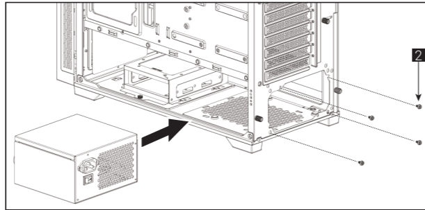
(2) Install PSU
