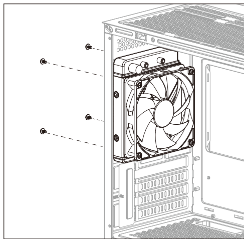
(7b) Install Rear Radiator
