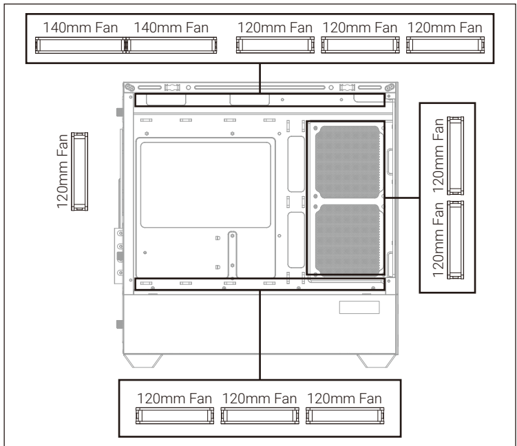
(6a) Install Top Fans
