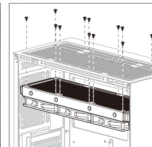
(7a) Install Top Radiator
