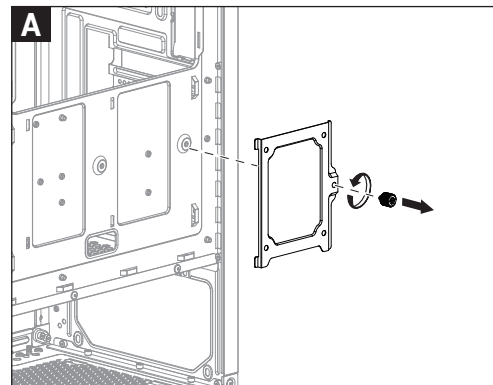
(5) Install 3.5" HDD x1
