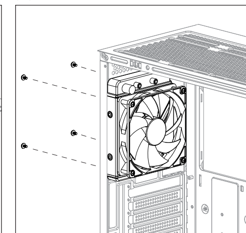
(7b) Install Rear Radiator
