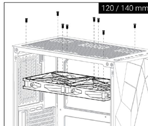
(6b) Install Top Fans
