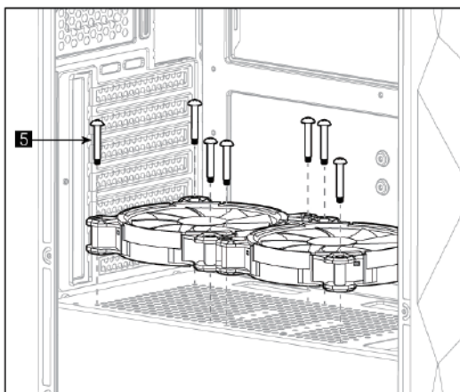
(6d) Install PSU Fans
