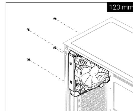
(7b) Install Rear Radiator
