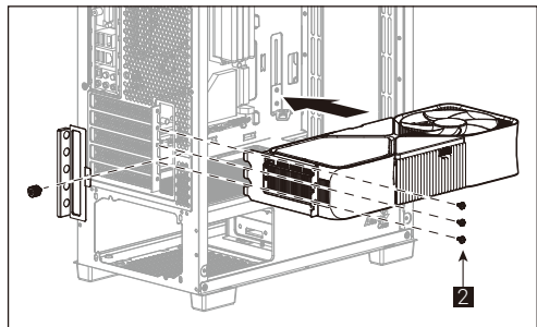
(3) Install VGA
