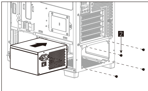
(2) Install Power Supply Unit
