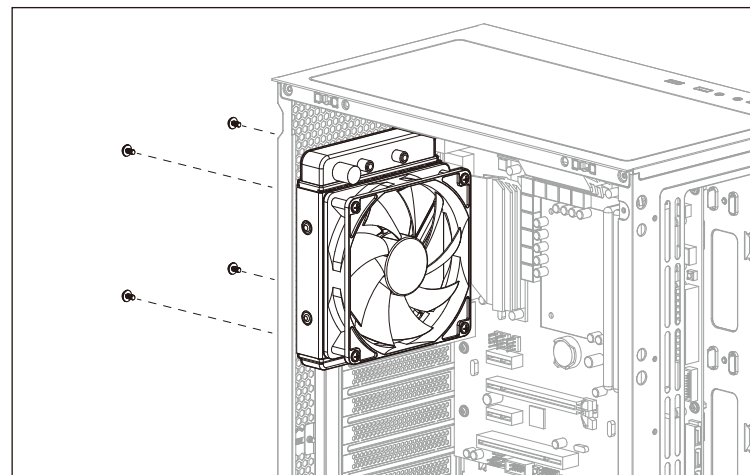
(6d) Install Rear Radiator
