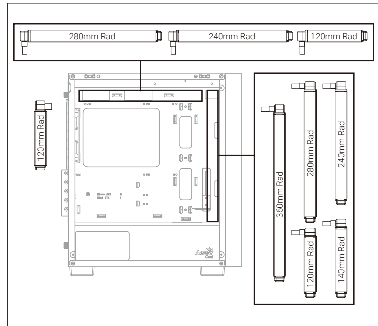
(6c) Install Top Radiator
