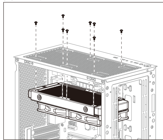
(6c) Install Top Radiator
