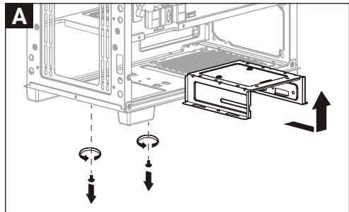
(4b) Install 2.5" SSD x1
