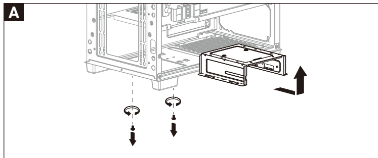
(5) Install 3.5" HDD x2
